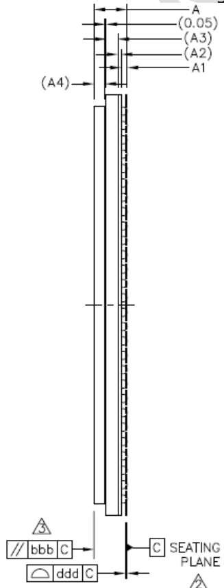
Fig. 2-3 RK3288 FCBGA636LD Package Side View
