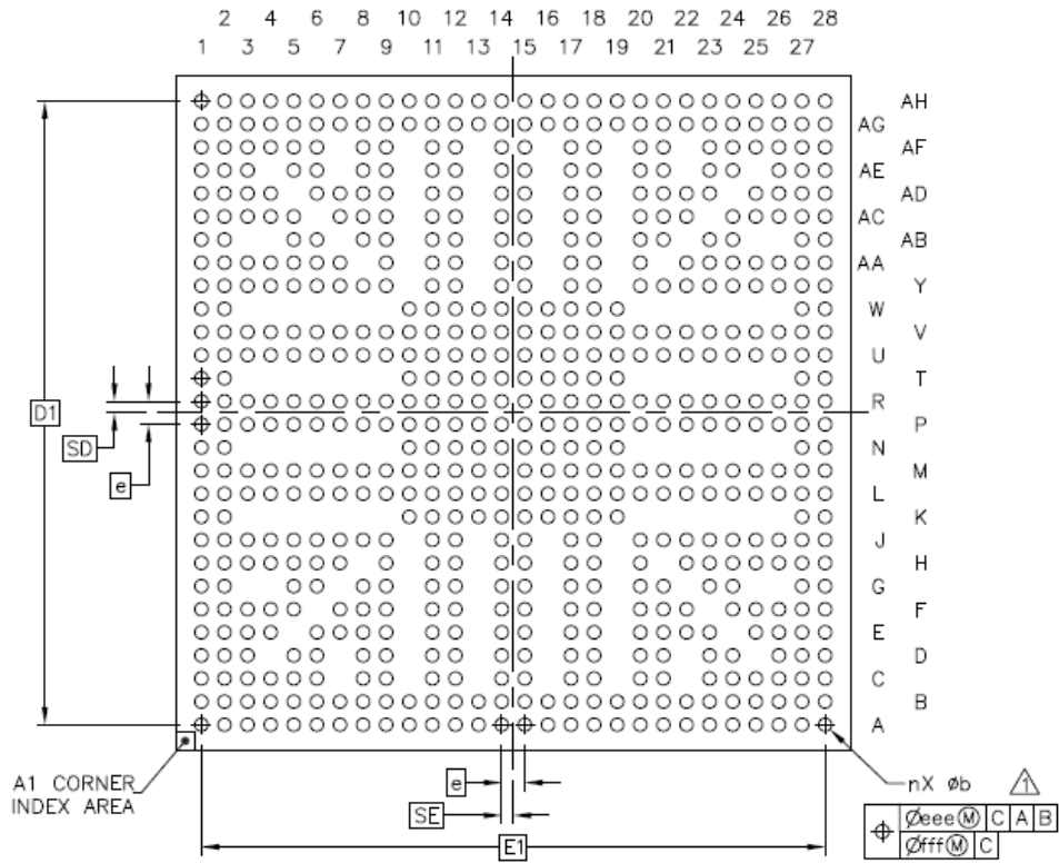
Fig. 2-2 RK3288 FCBGA636LD Package Bottom View
