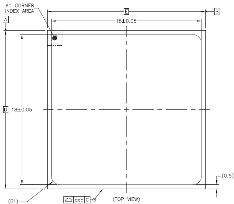
Fig. 2-1 RK3288 FCBGA636LD Package Top View
